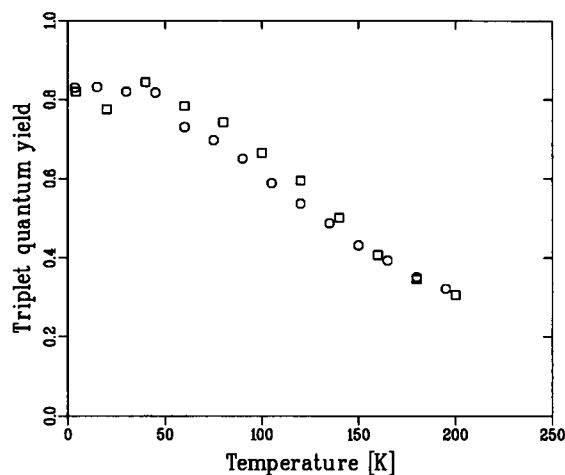
FIGURE 5 Absolute triplet quantum yields as a function of temperature, measured from 4 to 200 K (circles) and from 200 to 4 K (squares). The yields were calculated from the slope at zero intensity of saturation curves taken at 681 nm (see Material and Methods for details).
