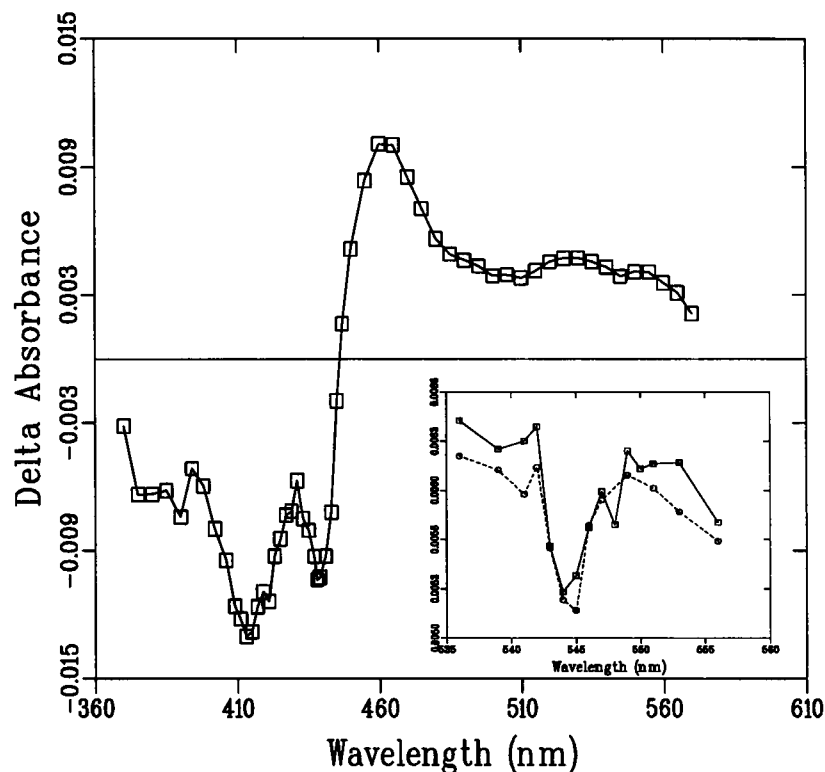
FIGURE 4 T - S absorbance difference spectrum from 370–570 nm at 77 K, constructed from the averaged amplitude 50–500 \mu s after the flashes. Inset : enlargement of Pheo Q_x region at 4 K (solid line) and 40 K (dashed line).
